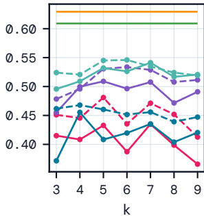
RMSE (%)
