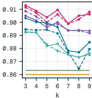
Kendall \tau
