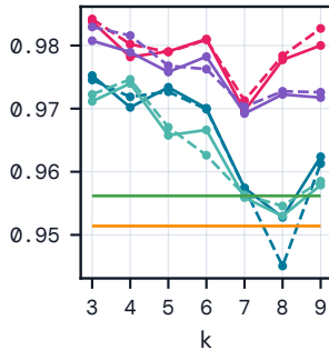
Spearman \rho
